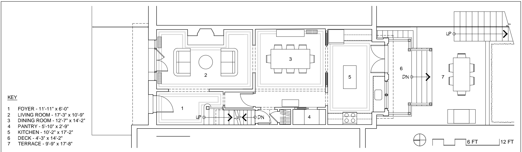
FIRST FLOOR PLAN - AFTER
