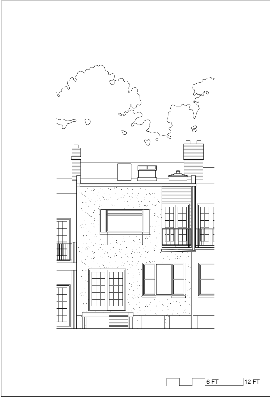
SOUTH ELEVATION - BEFORE
